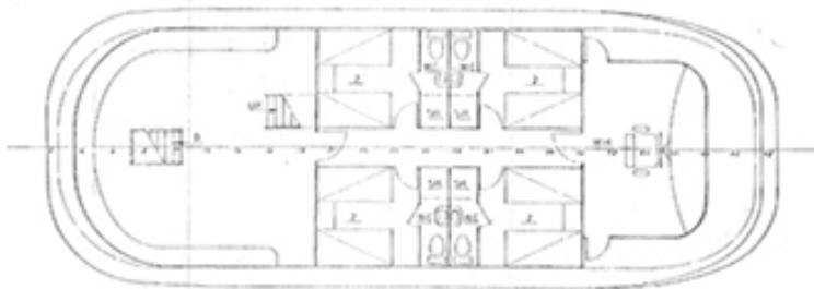
WHEEL HOUSE DECK
